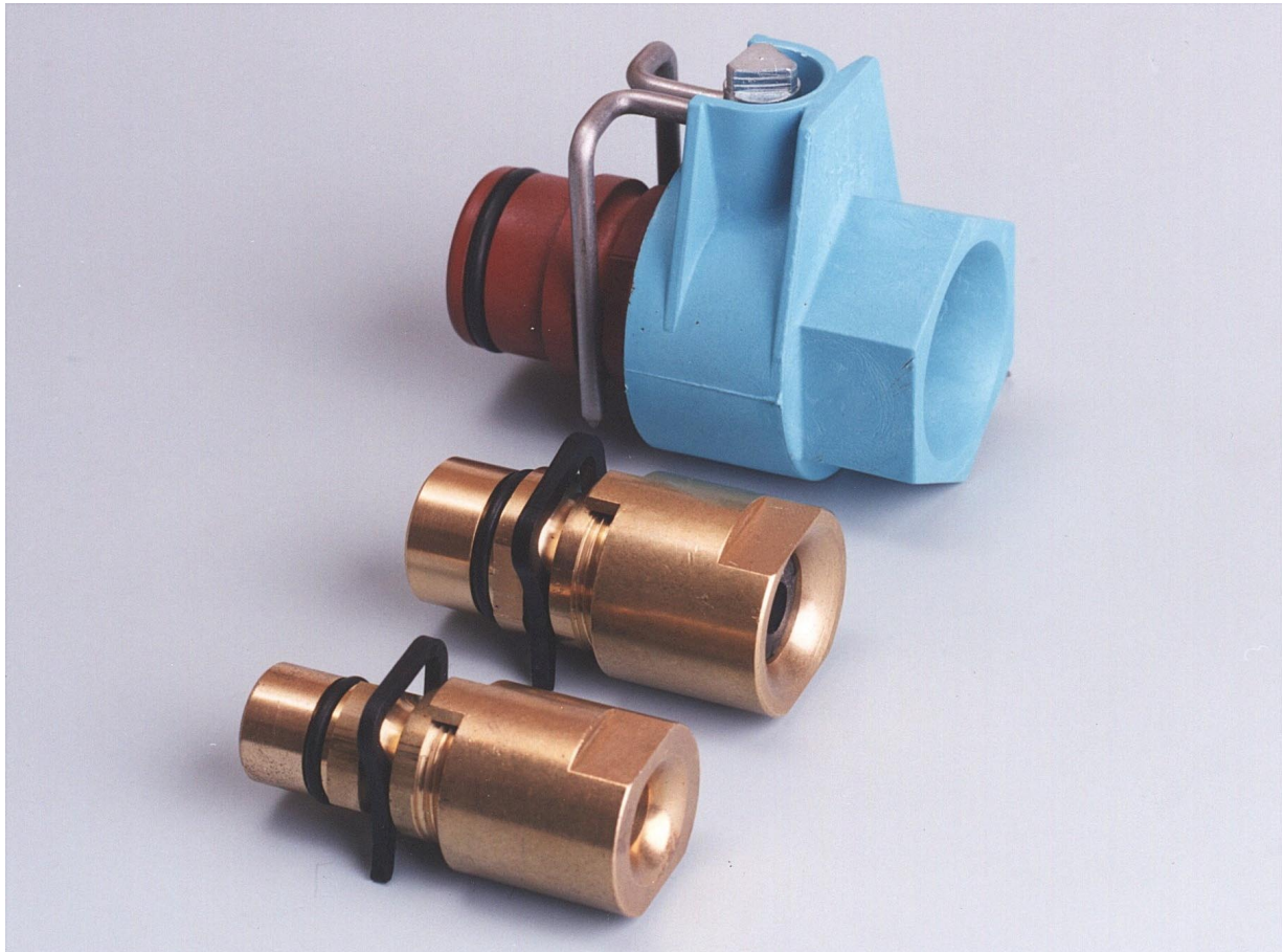
Photo: Quick-connectors of sizes HA-LSA i 1; HA-LSA i 2 and HA-LSA-3 (i)
